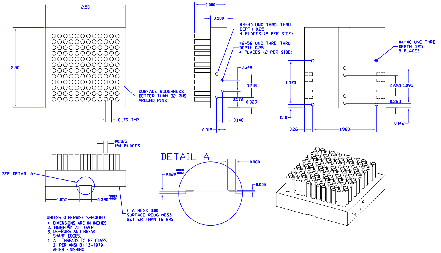
Heat Sink Drawing
